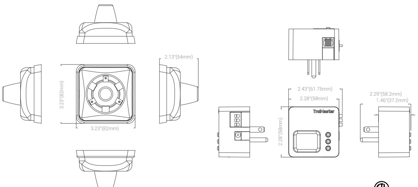
AS-1 CO2 Alarm Station Set
