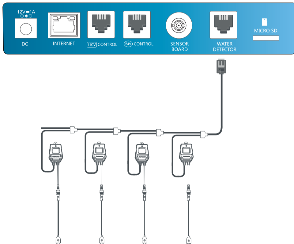
Water Detectors
